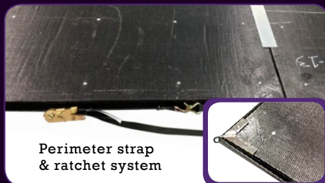
4' x 8' Floor Panel
